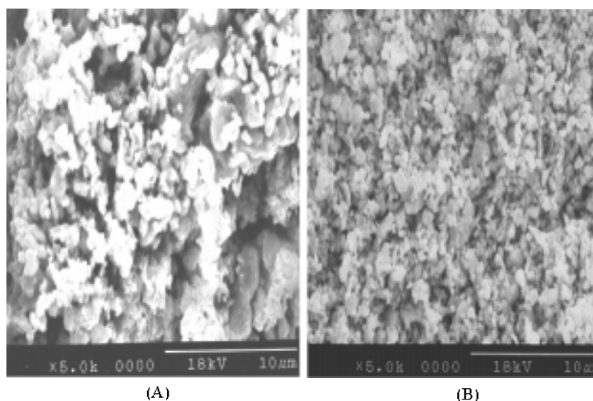
Fig. 4. Scanning electron microscope of \text{La}_2\text{Ti}_2\text{O}_7 prepared with different grinding methods. (A) Dry grinding method, (B) Wet grinding method
