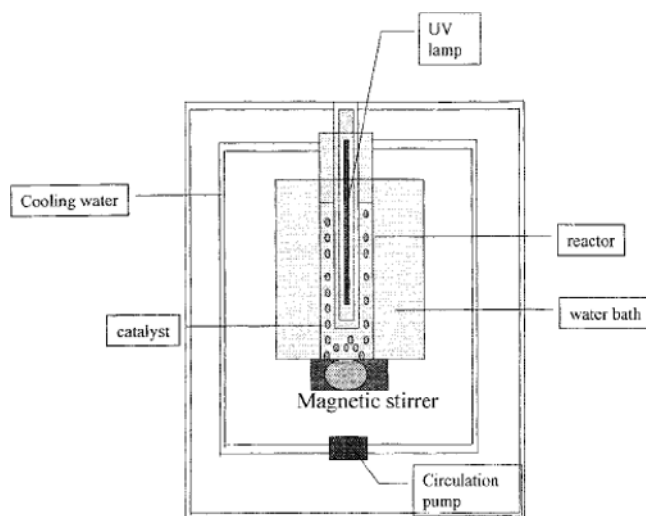
Fig. 3. A closed circulation reaction system for photocatalytic water splitting.
