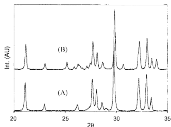
Fig. 11. XRD patterns of \text{La}_2\text{Ti}_2\text{O}_7 from different \text{La} precursors. (A) \text{La}_2\text{O}_3 , (B) \text{La}_2\text{O}_3 from \text{La}_2(\text{CO}_3)_3
